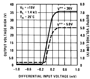
Transfer Function
